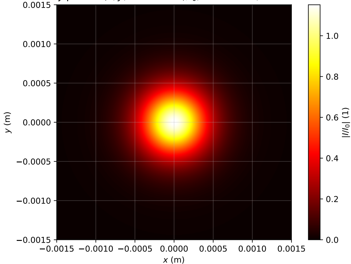
Intensity profile I(x, y, z = 2.786m)/I_0 , \text{Pin}=0.8\text{Pcr} , artificial time
